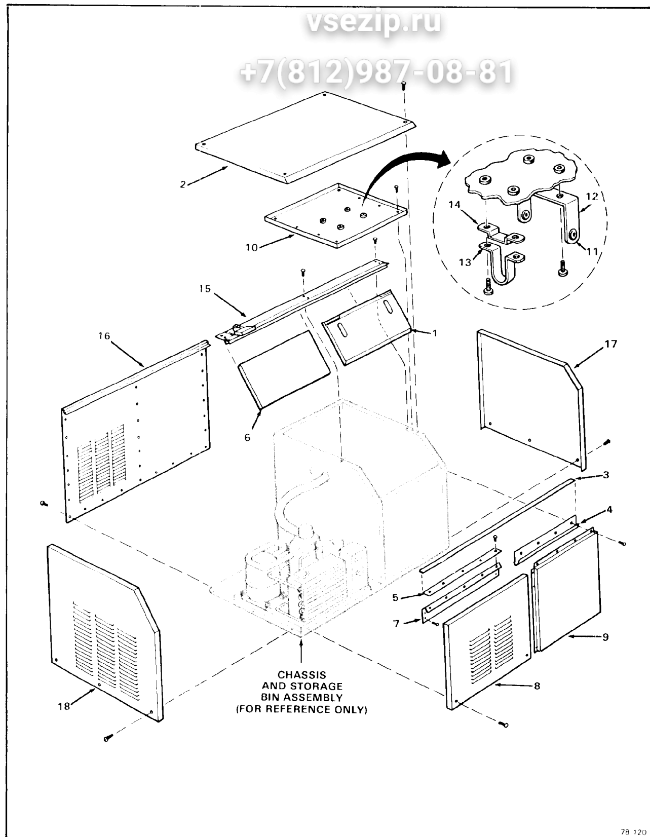
Figure 8-1. AF-430 Cabinet.
