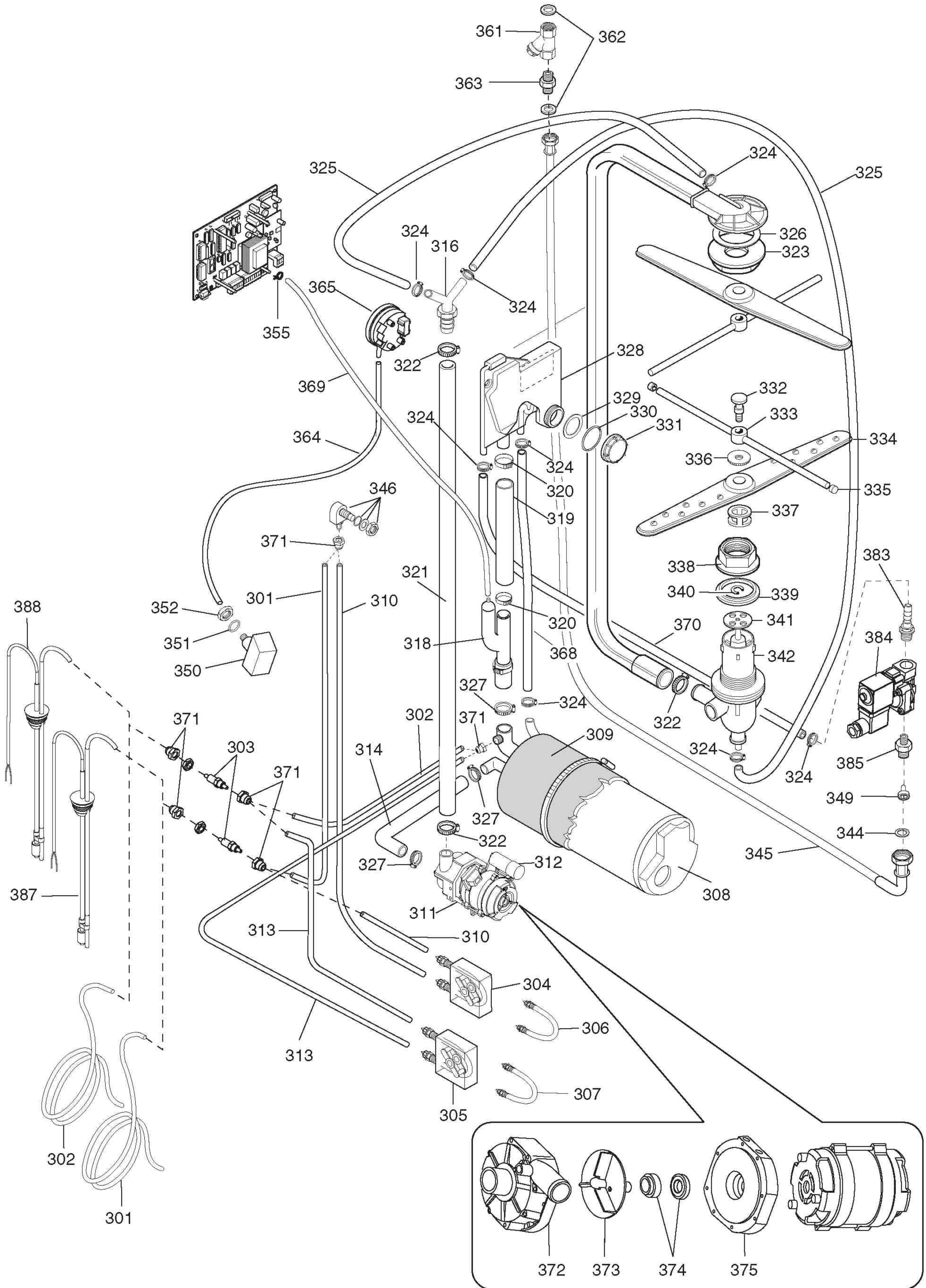
III. 611004p4usa Circuito idraulico / Hydraulic circuit
