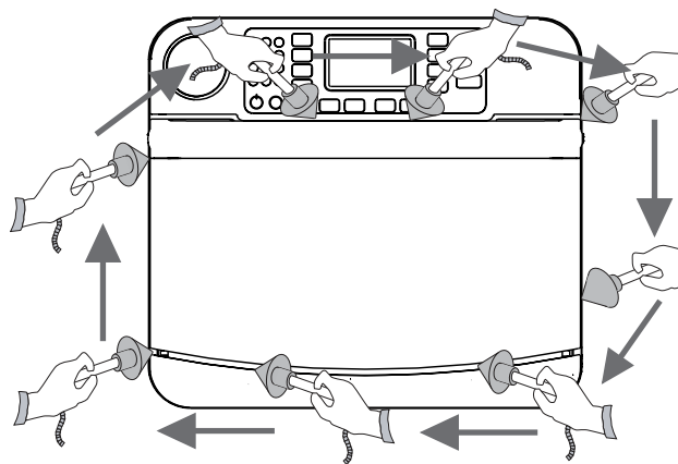
Figure 39: Measure for Microwave Leakage
