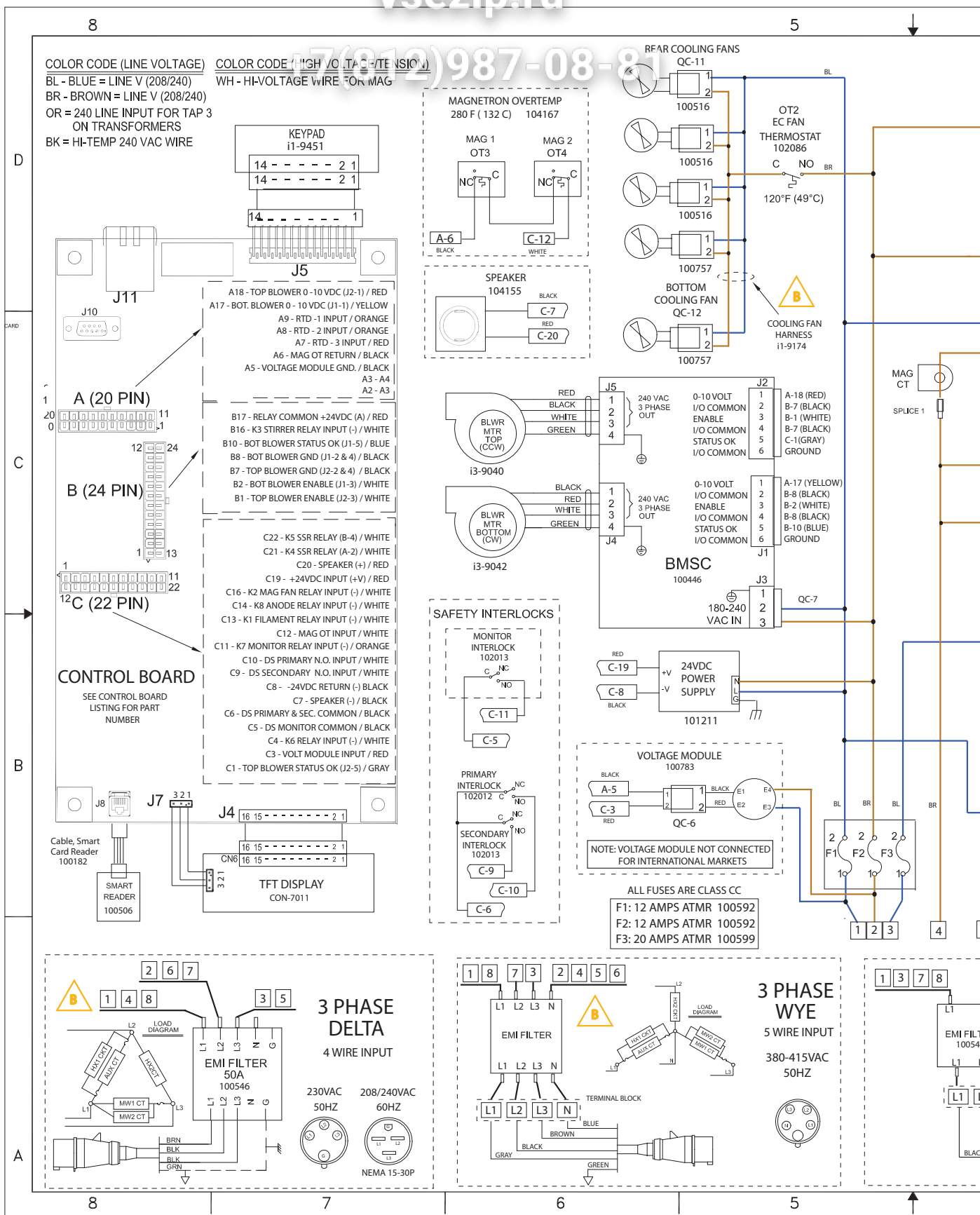
Figure 38: Oven Schematic
