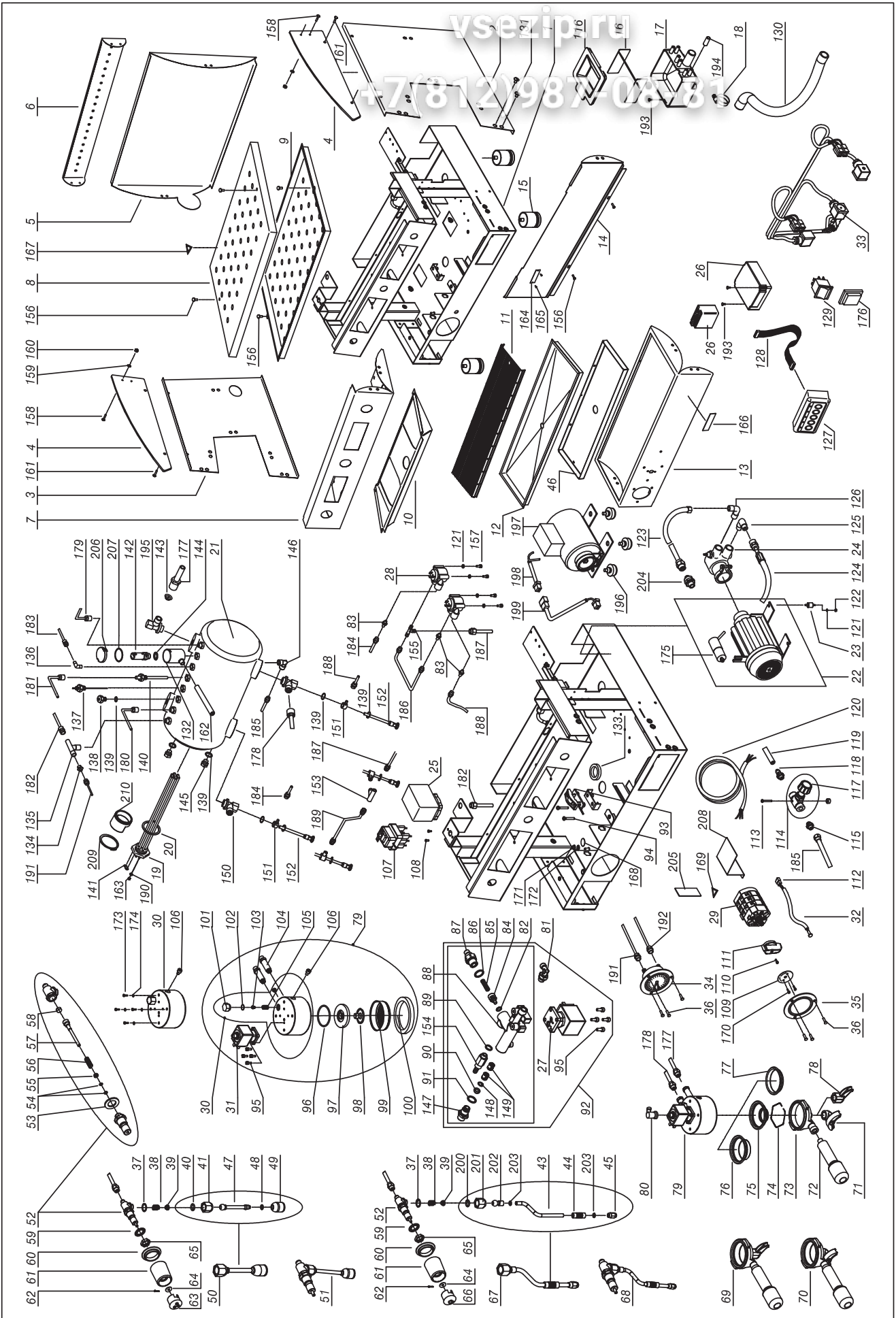
Exploded view CAPRI DELUXE update 07-13
