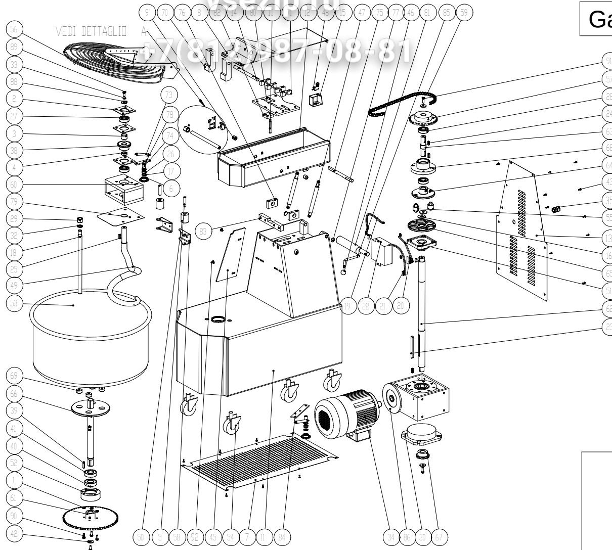
Impastatrice a spirale TSVX60 (vasca estraibile) - Spiral dough mixer TSVX-60 (extractable bowl)
