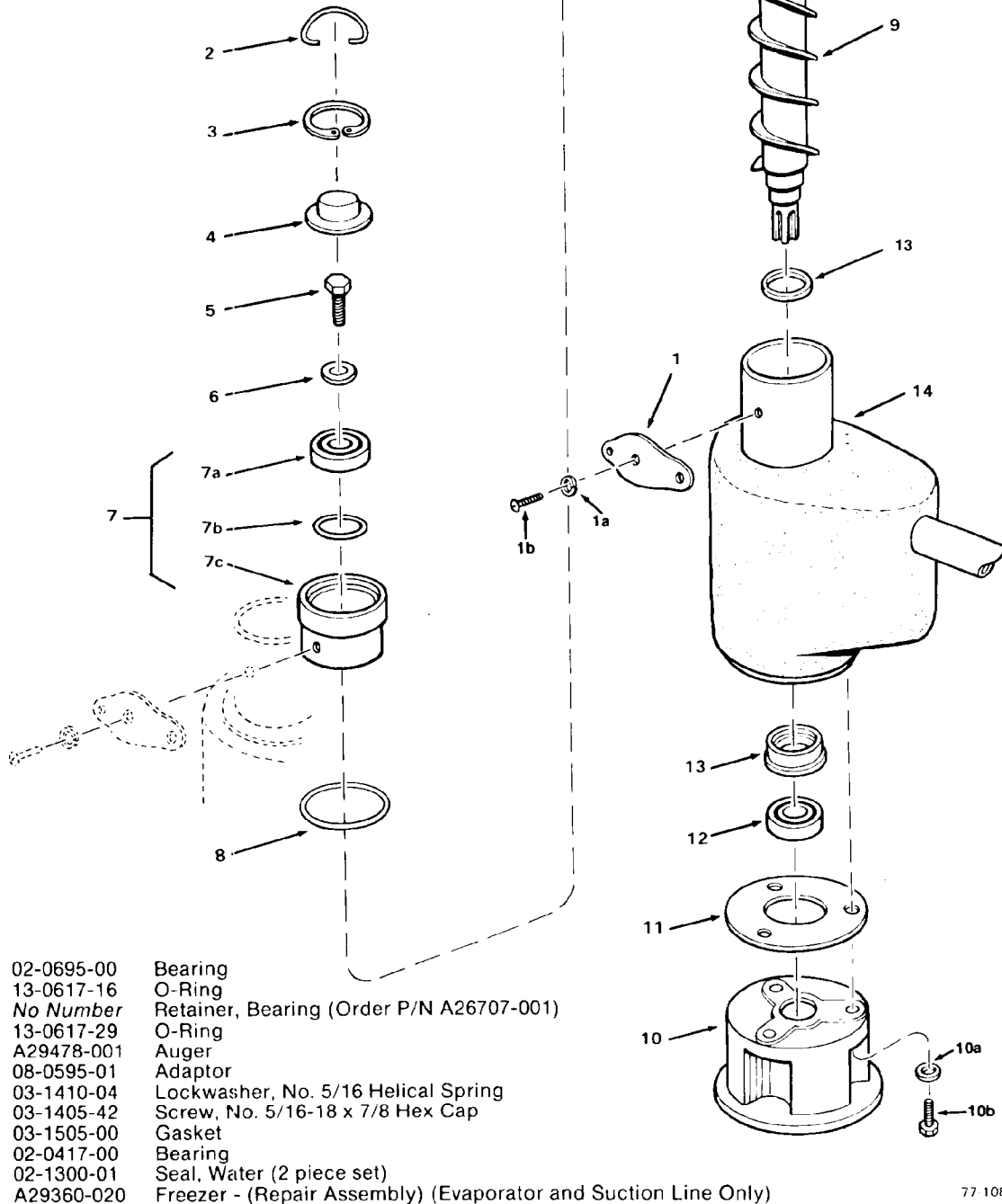
Figure 8-5. Freezer Assembly.
