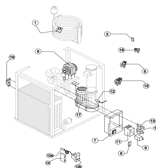
ELECTRIC PARTS
