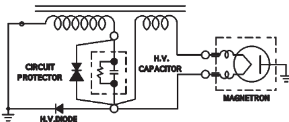
HV CIRCUIT ( 2 PLACES)
