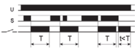
FZ08: Fixed pulse (0.5s) delayed
