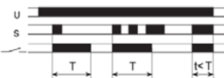
FZ06: Power is permanently applied to the timer
