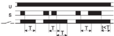
FZ03: Symmetrical recycling: ON start
