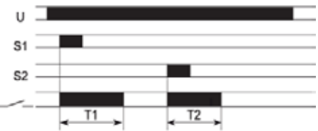
FZ37: Signal OFF delay with Start/ Stop pushbutton
