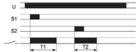
FZ37: Signal OFF delay with Start/ Stop pushbutton
