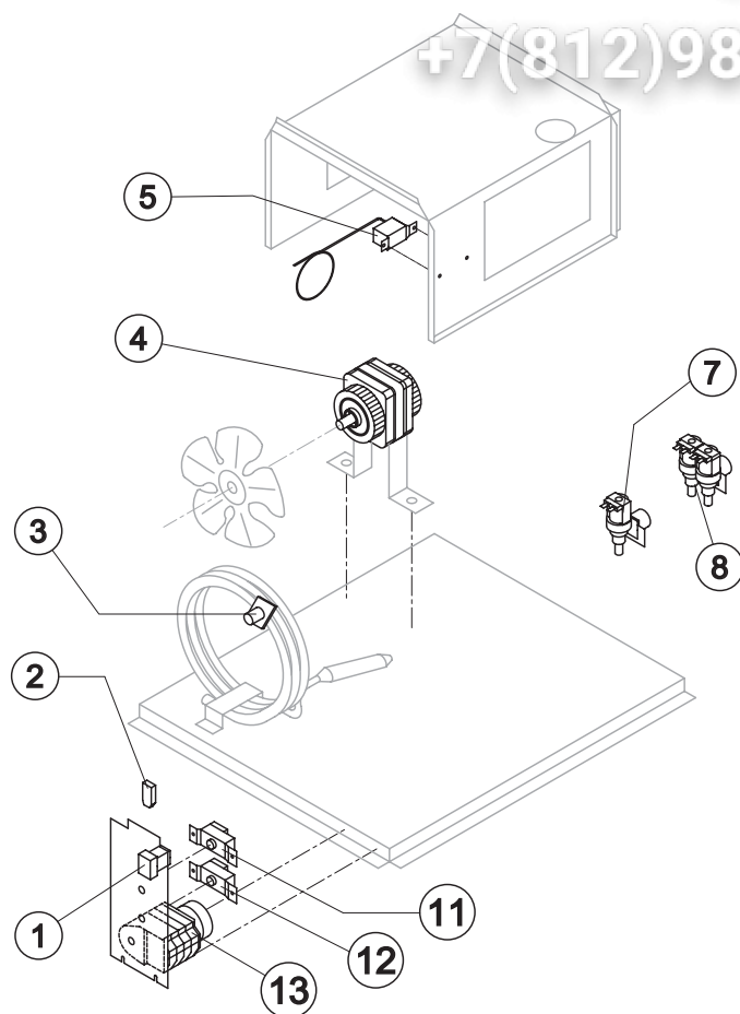
Ref. 7* - 1 Way- Water Inlet Valve
