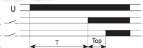
FZ27: 1 relay ON delay, 1 relay OFF delay
