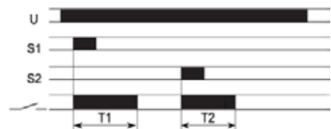
FZ32: Clock generator - Start after impulse
