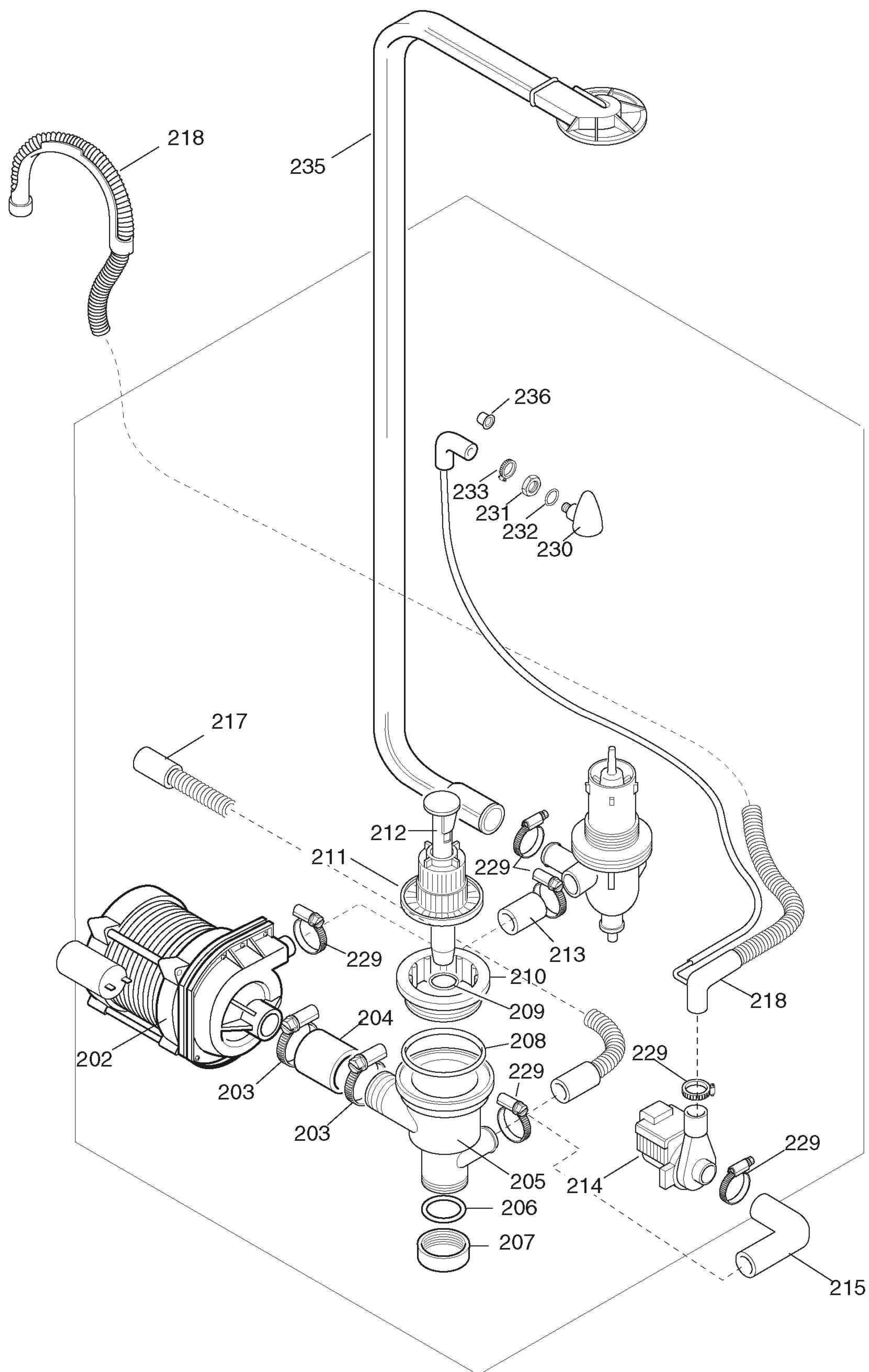
ill. 611002p3 Componenti idraulici / Hydraulic components
