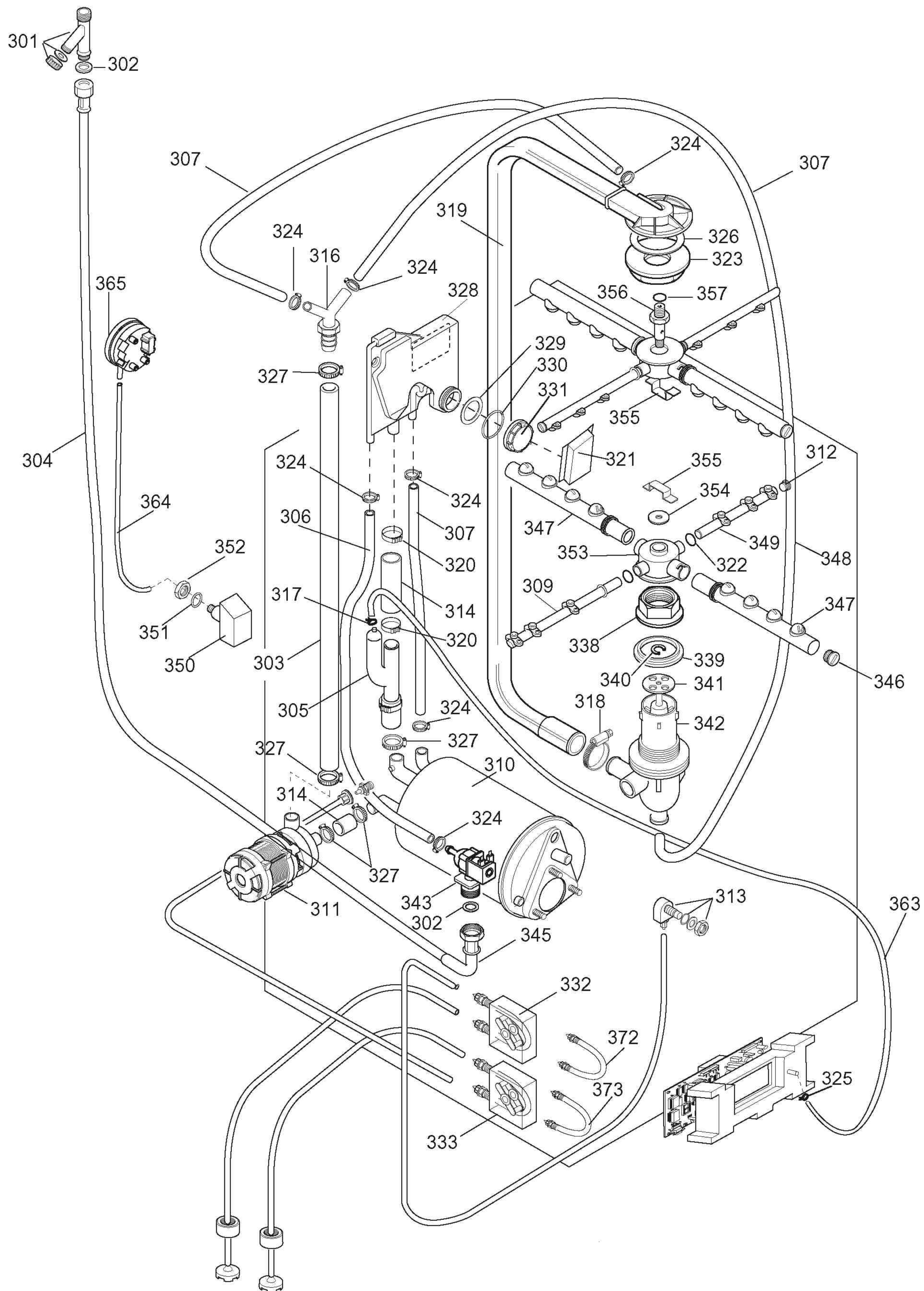
ill. 611002p4 Circuito idraulico / Hydraulic circuit
