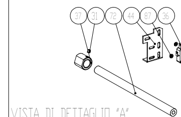
Impastatrice a spirale TSVX60 (vasca estraibile) - Spiral dough mixer TSVX-60 (extractable bowl)
