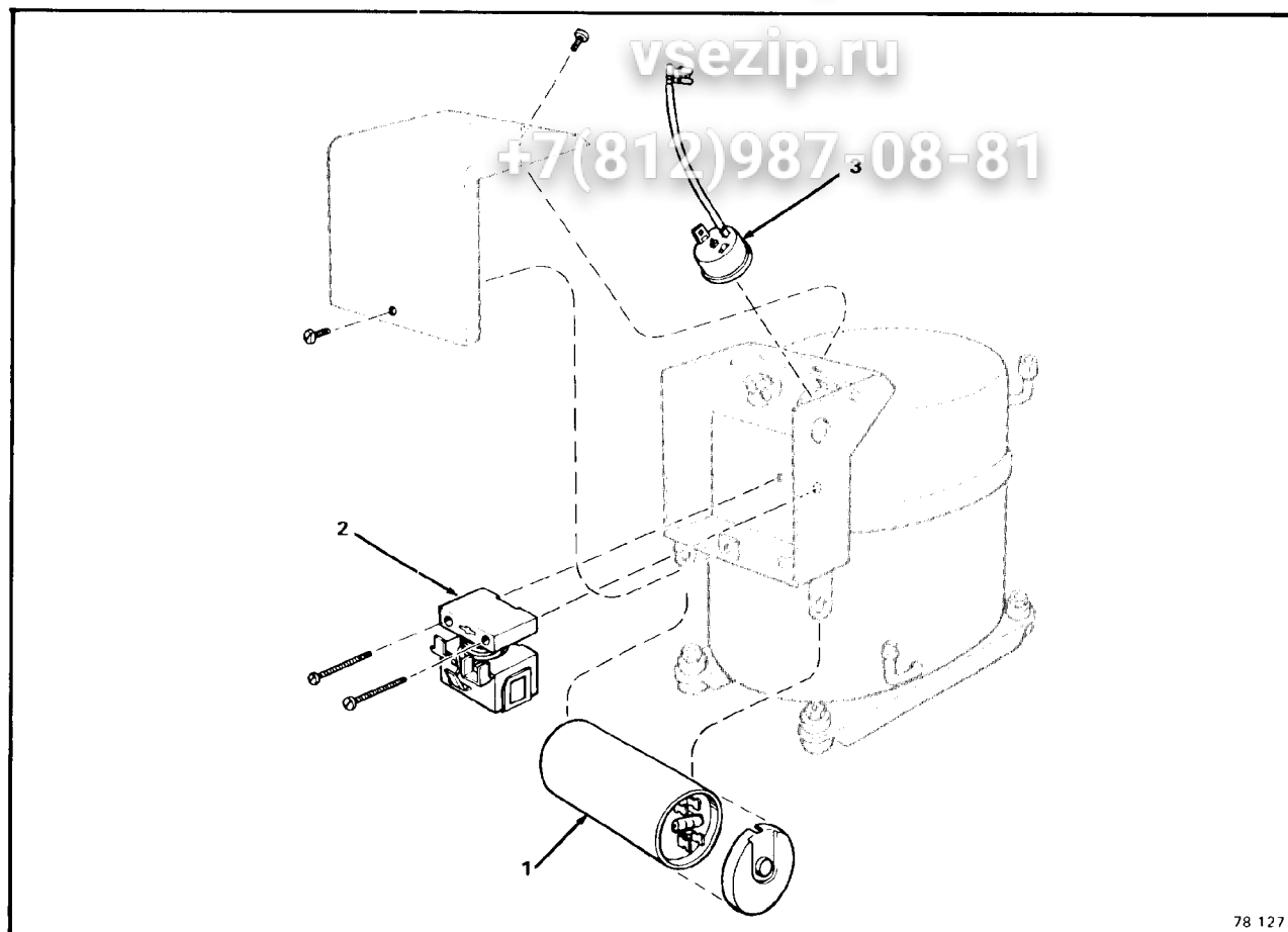
Figure 8-4. Compressor Assembly
