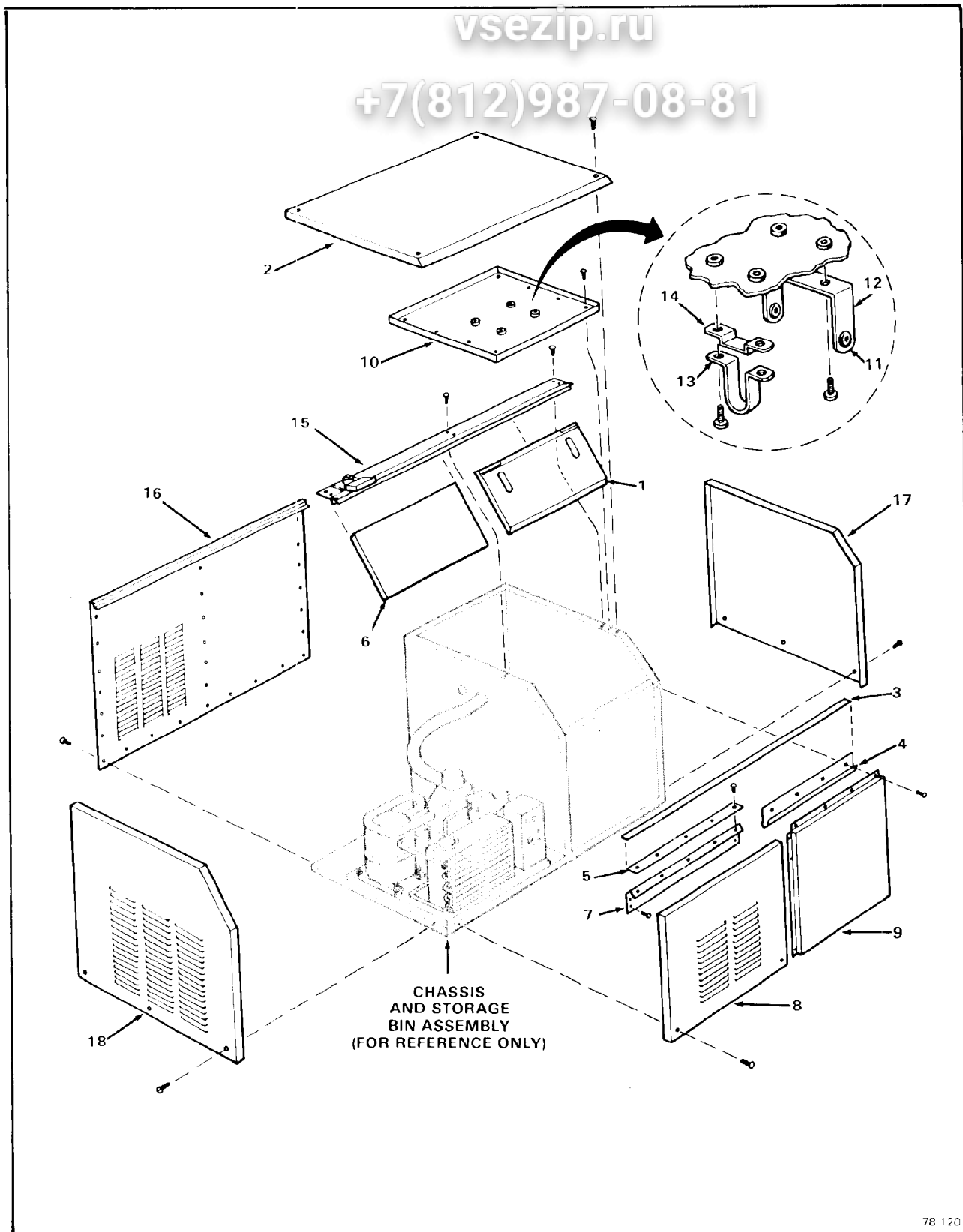
Figure 8-1. AF-730 Cabinet
