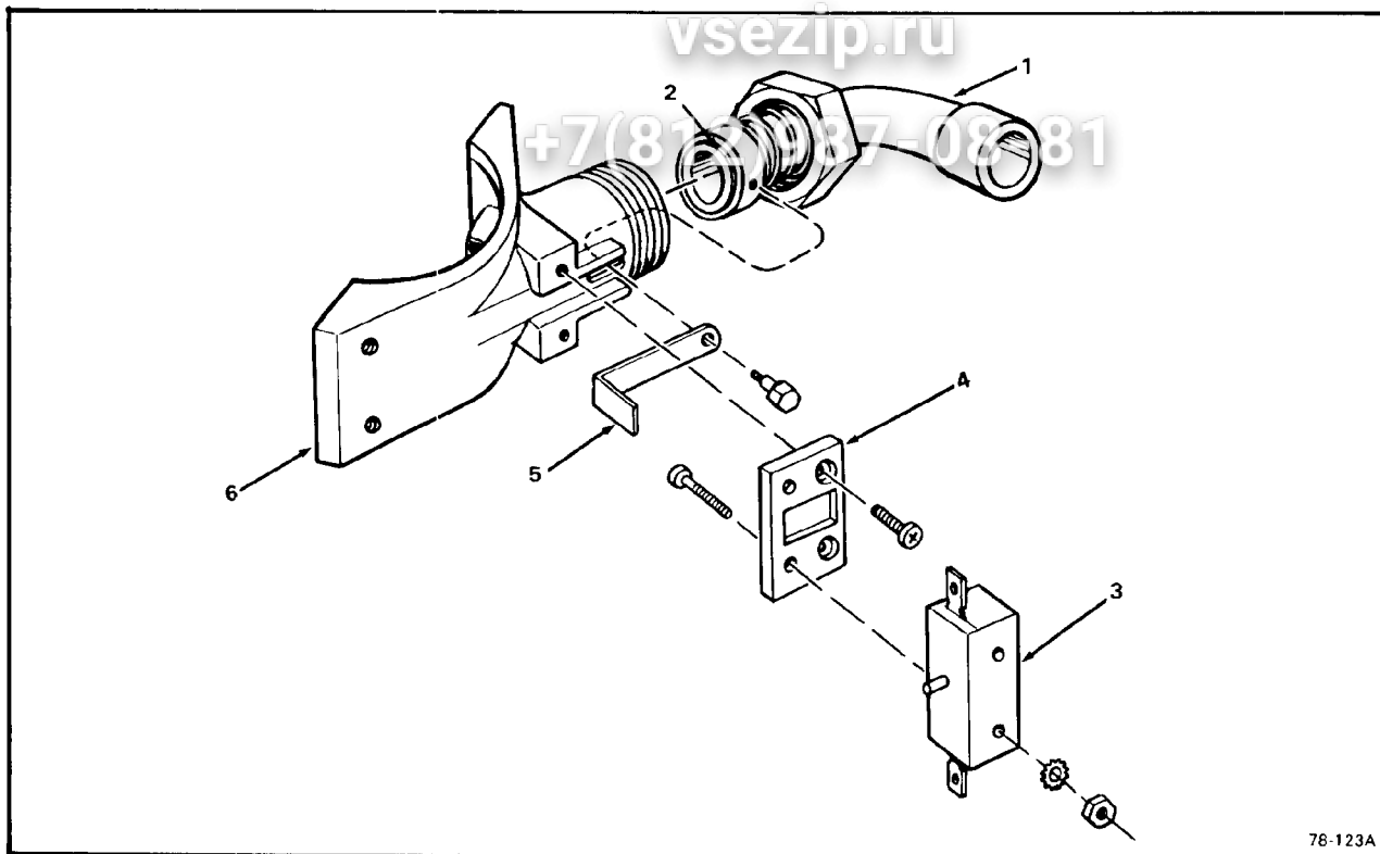
Figure 8-5. Spout Assembly.
