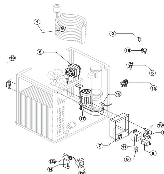
ELECTRIC PARTS
