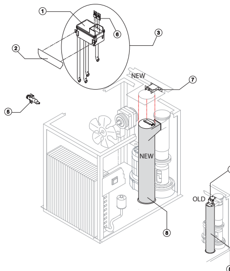
HYDRAULIC CIRCUIT
