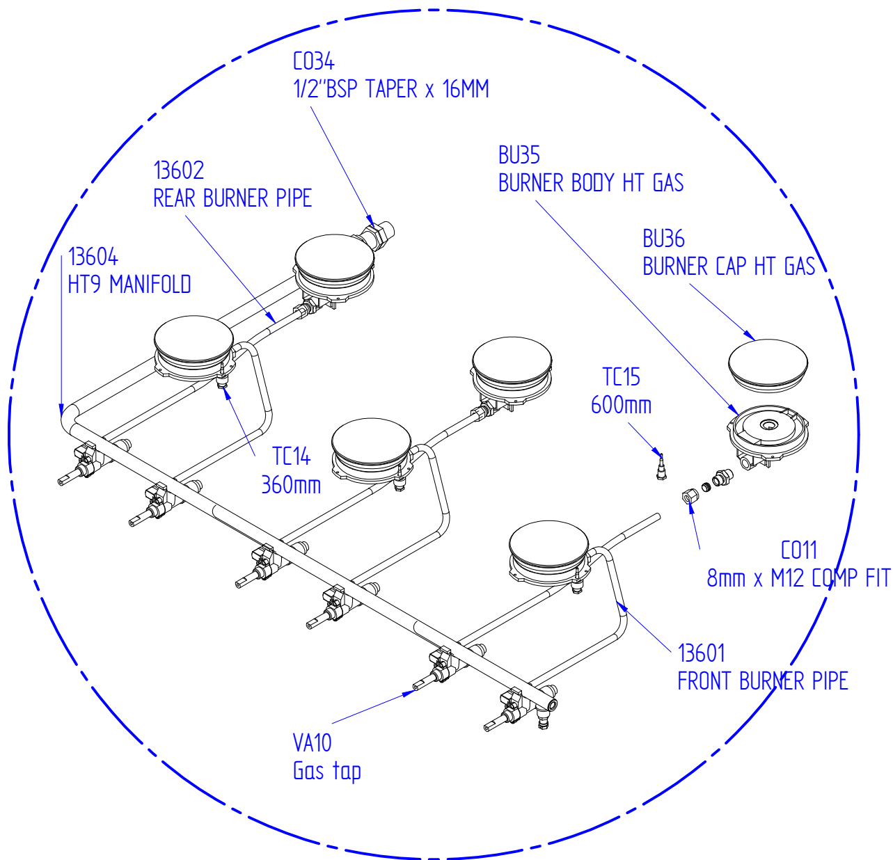
DETAIL A
