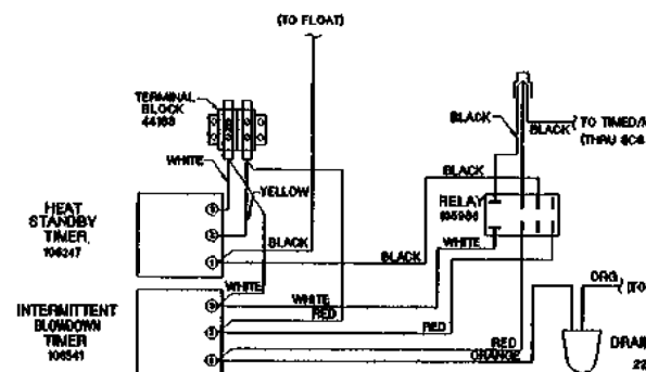
INTERMITTENT BLOWDOWN OPTION
