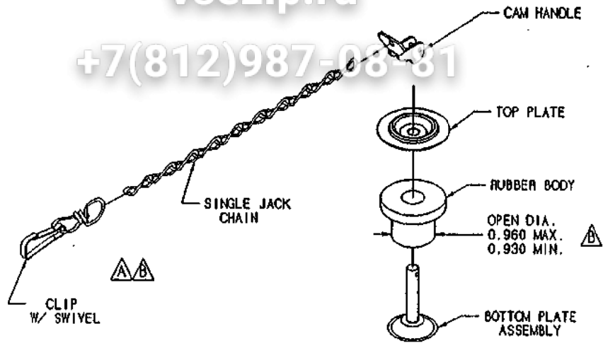
EXPLODED VIEW
