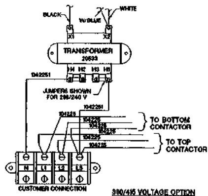
380/415 VOLTAGE OPTION
