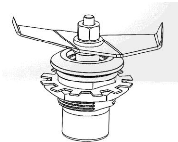
Cutter Assembly 98650
