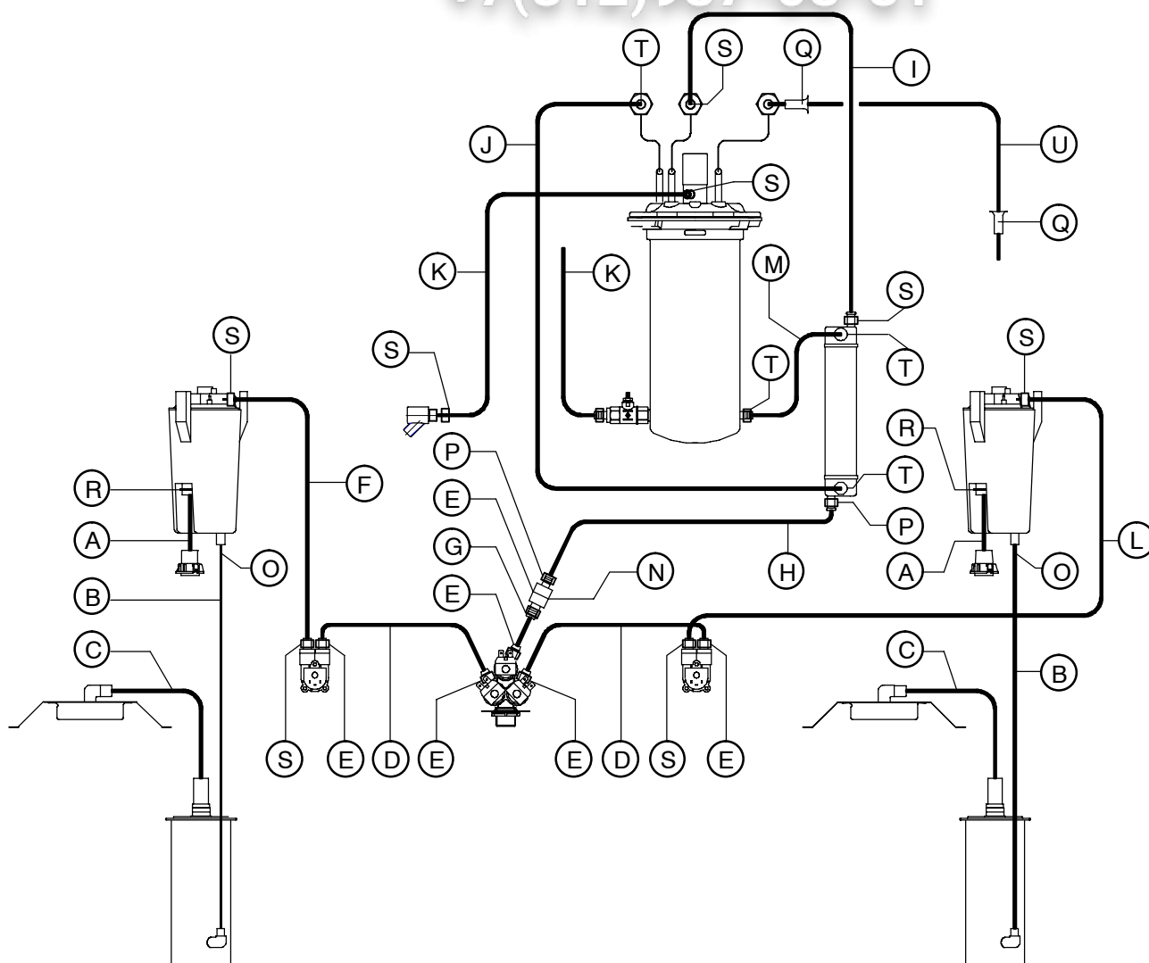
Fig. 3 Tube diagram BFT322-001
