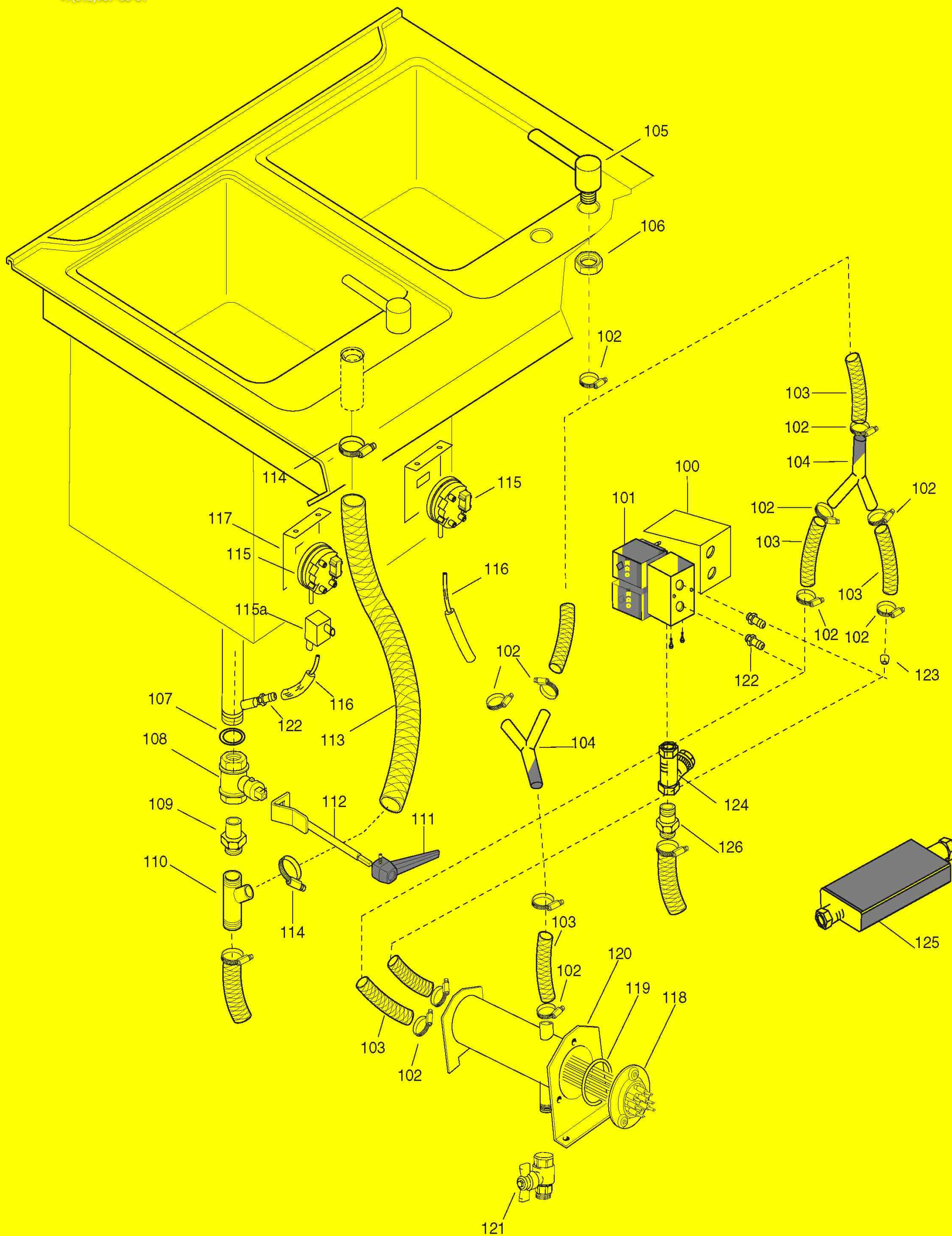
Cuocipasta Gas N900 Gas Pasta Cooker N900
