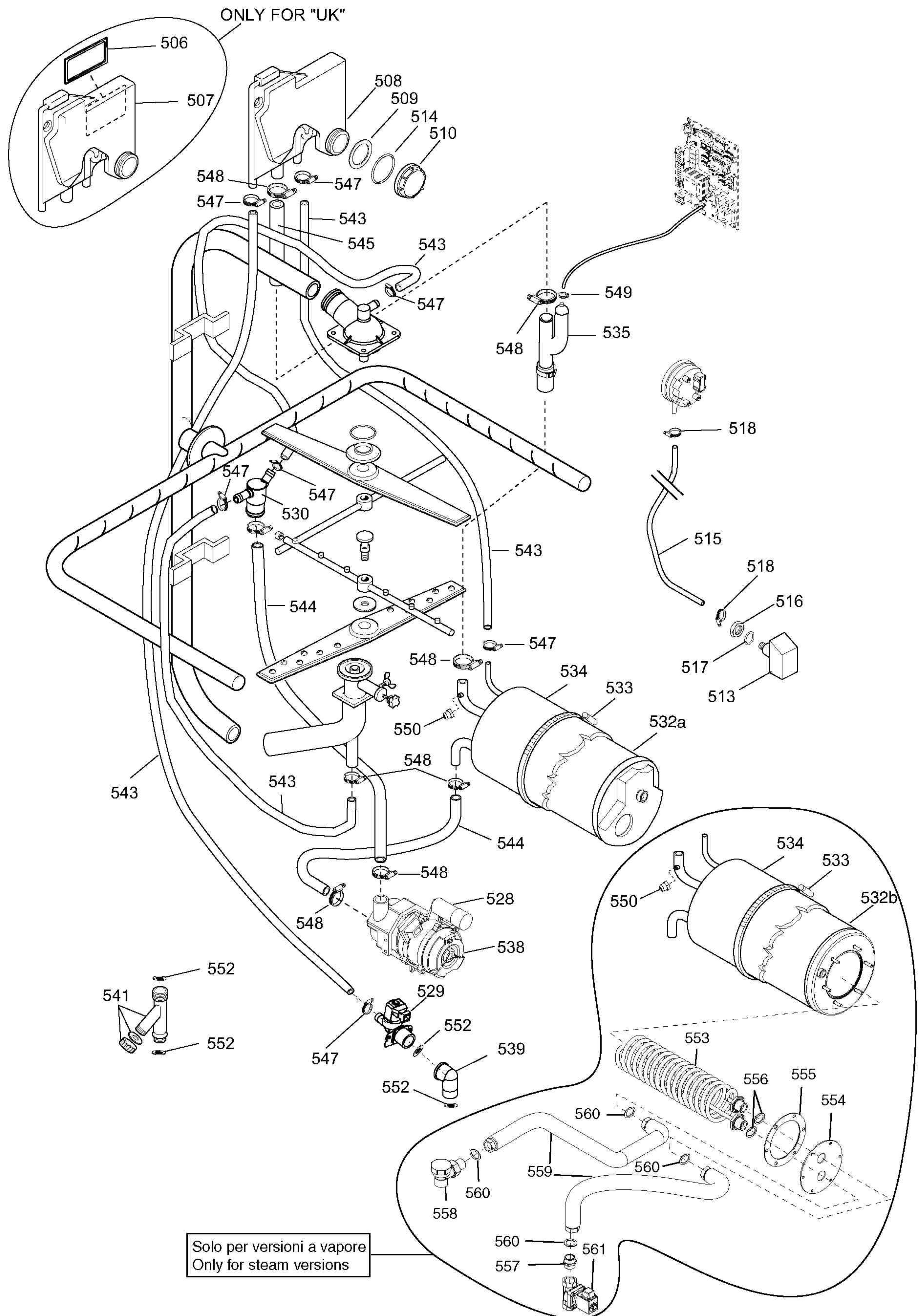
ill. 681002p5A_A Circuito idraulico * / Hydraulic circuit *
