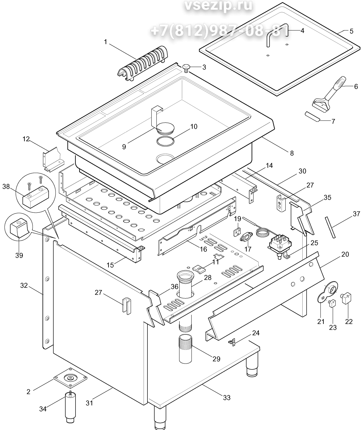
GAS BRATT PAN FIXED TANK BRASIERA GAS A VASCA FISSA
