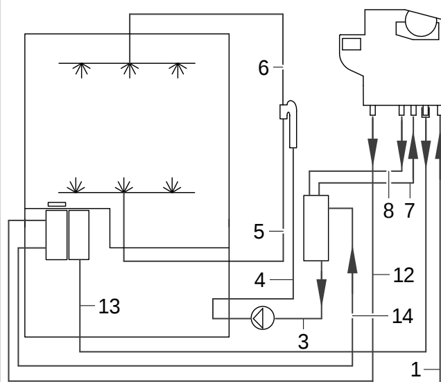
Water softener
