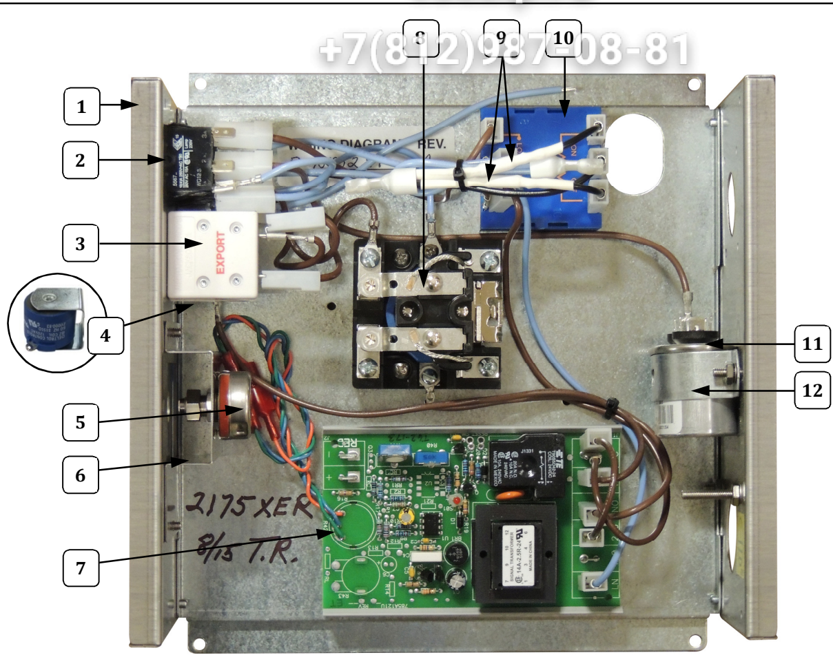
Control Panel Interior (Model 2175XER shown)
